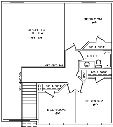
UPPER LEVEL (OPT 9'-0" CEILINGS)
