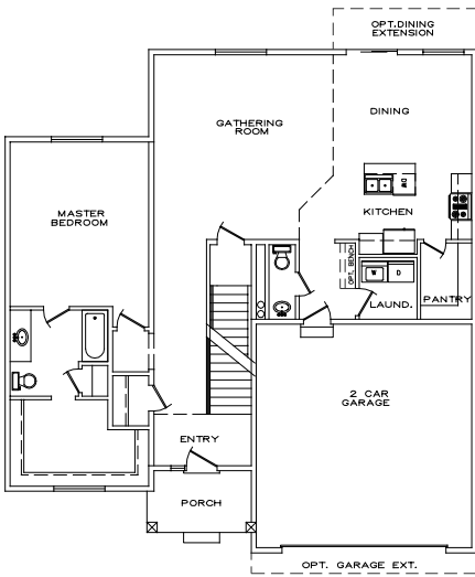
MAIN LEVEL (OPT 9'-0" CEILING)
