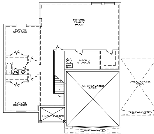
UNFINISHED BASEMENT (OPT 9'-0" WALLS)
