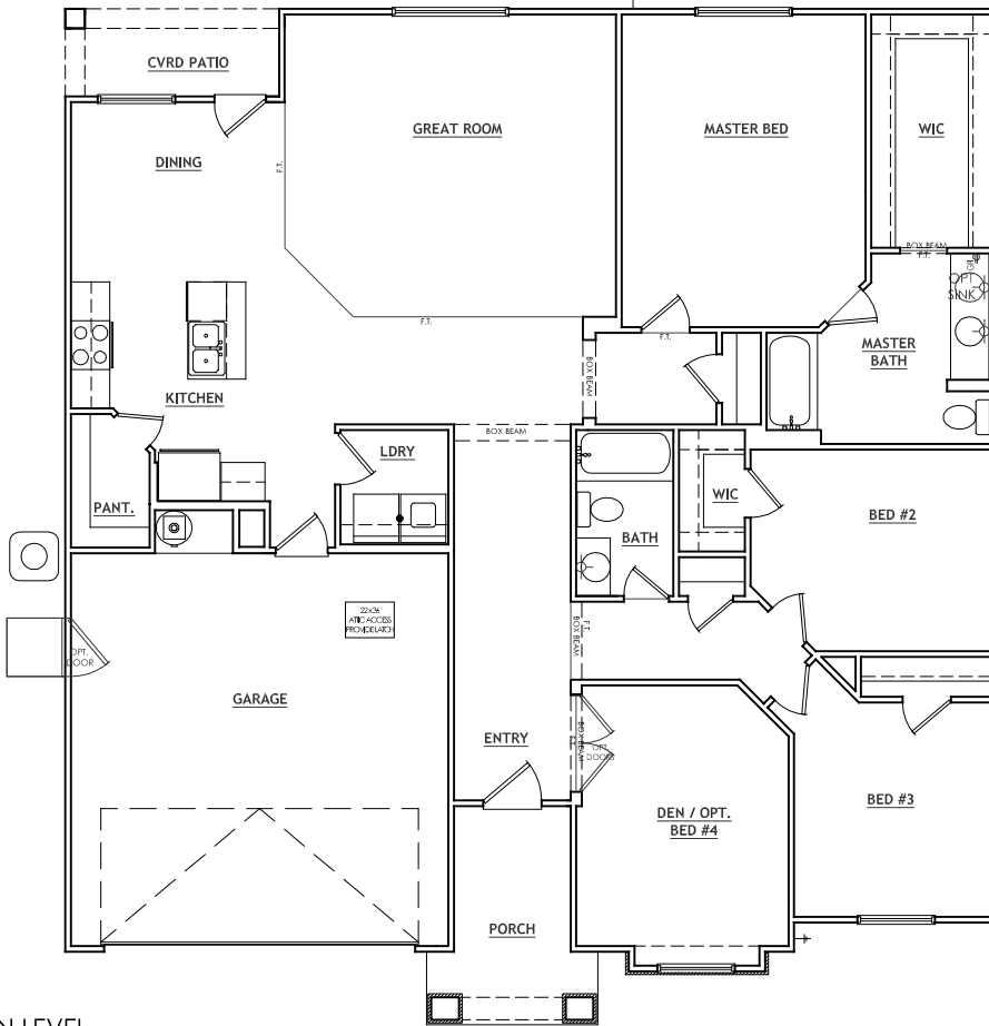
MAIN LEVEL (OPTIONAL 9'-0" CEILING)
