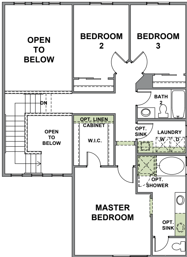
SECOND FLOOR PLAN 902 Sq.Ft.
