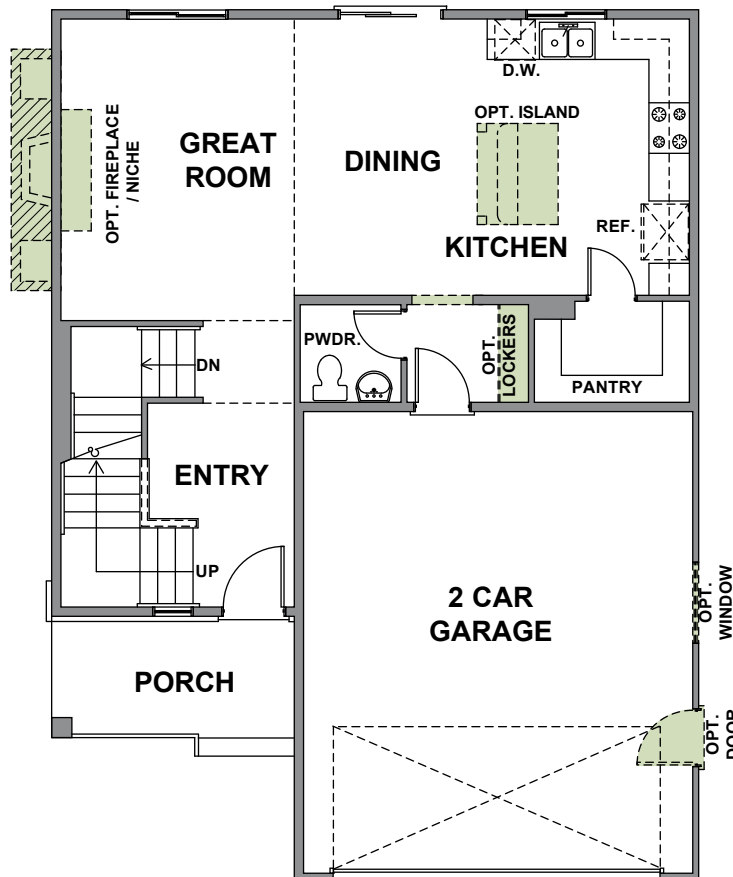
FIRST FLOOR PLAN 762 Sq.Ft.
