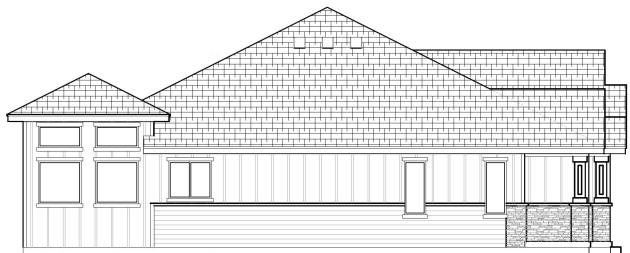
LEFT ELEVATION
