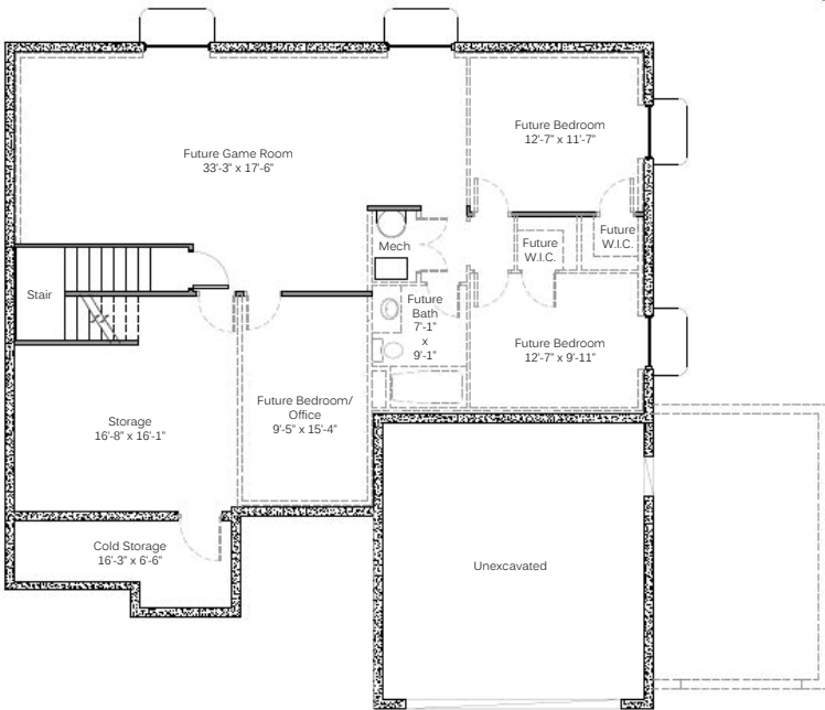
BASEMENT FLOOR
