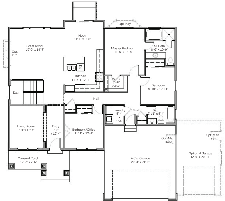
MAIN FLOOR
