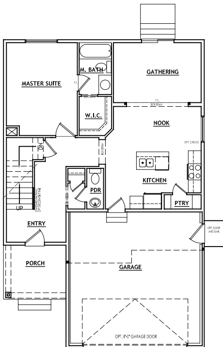
MAIN LEVEL (OPT. 9' CEILINGS)
