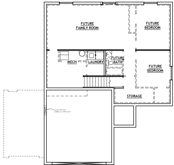
UNFINISHED BASEMENT (OPTIONAL 9'-0" WALLS)
