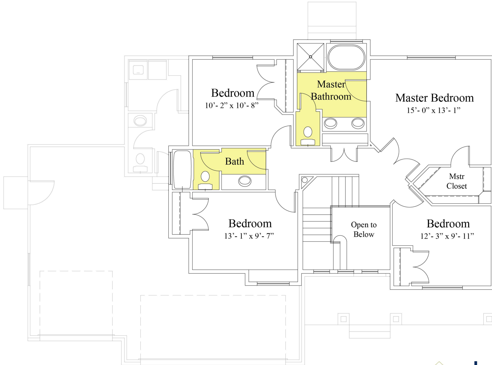
Floor Plan: Carter (TS2000) Upper Floor
