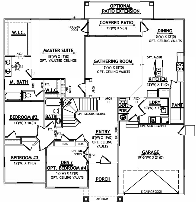
MAIN LEVEL (OPT. 9' CEILINGS)
