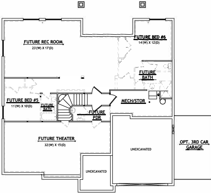
BASEMENT LEVEL
