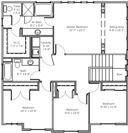
UPPER FLOOR
