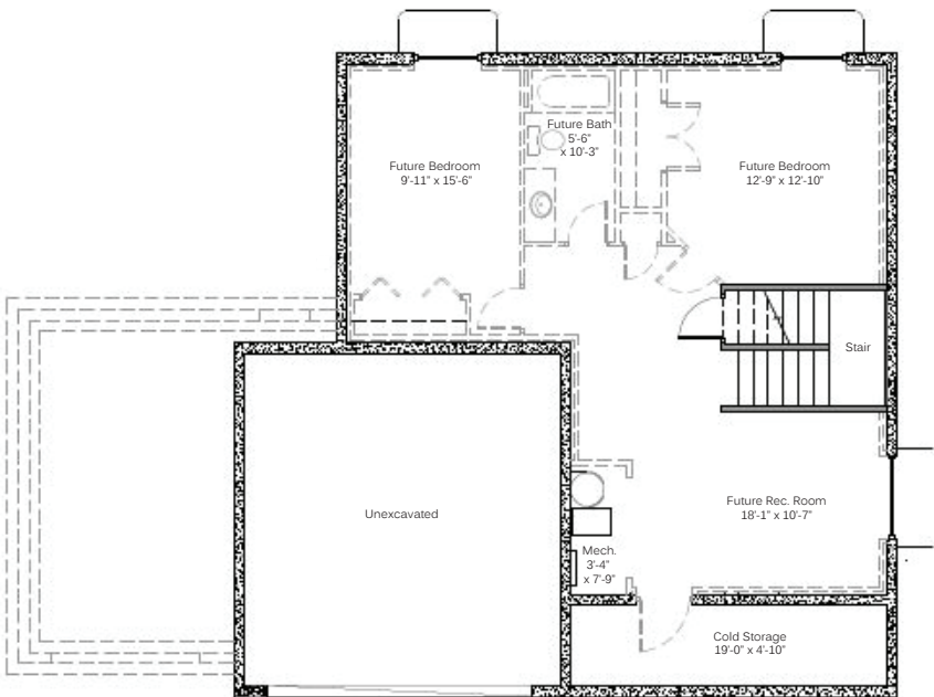
BASEMENT FLOOR
