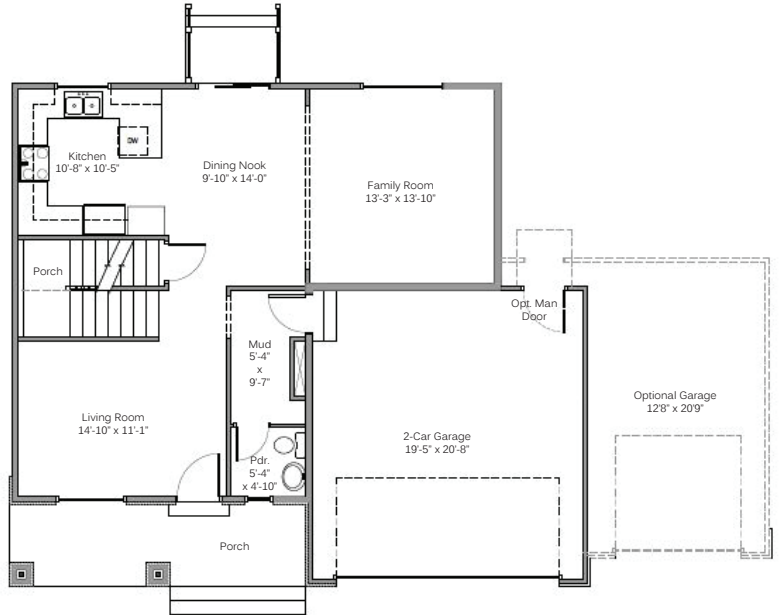
MAIN FLOOR
