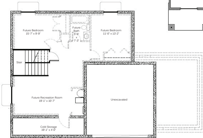
BASEMENT FLOOR
