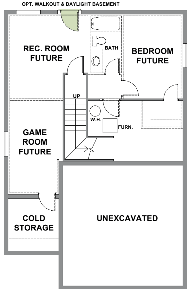
BASEMENT FLOOR PLAN 65 Sq.Ft. Finished 674 Sq.Ft. Unfinished
