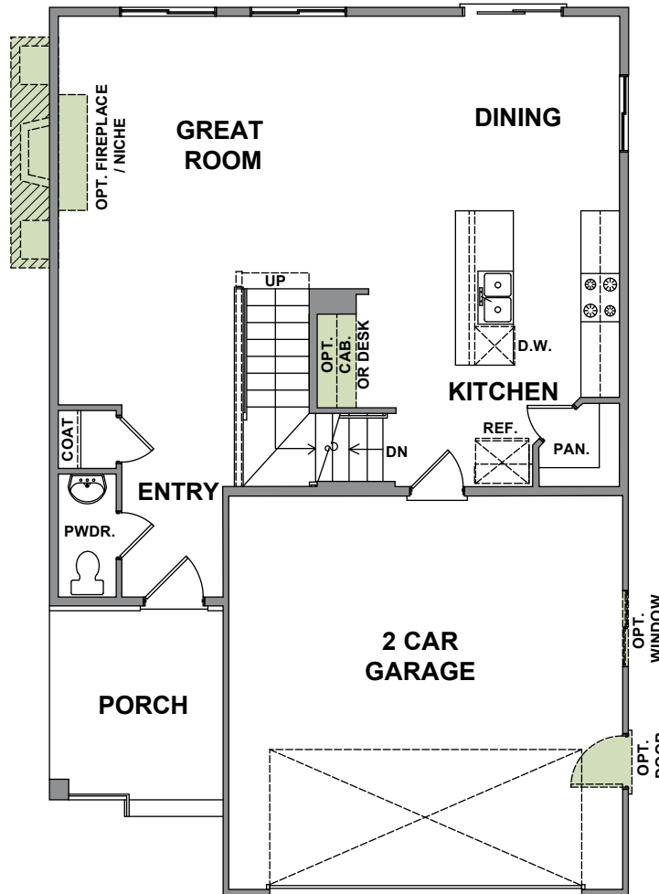
FIRST FLOOR PLAN 812 Sq.Ft.
