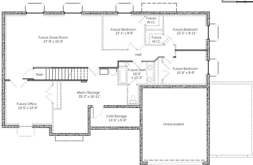
BASEMENT FLOOR
