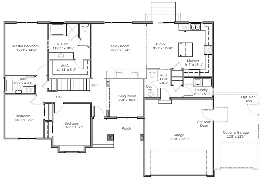
MAIN FLOOR
