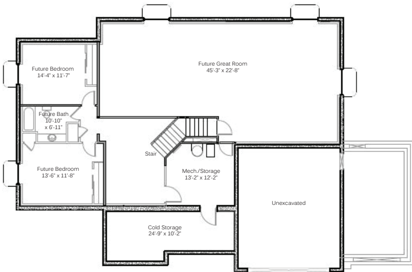
BASEMENT FLOOR
