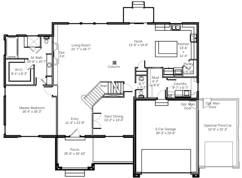
MAIN FLOOR
