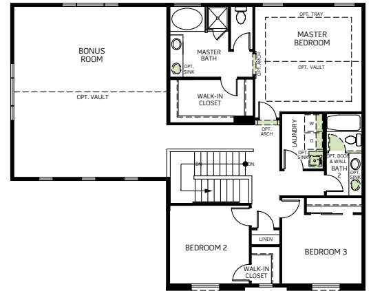
SECOND FLOOR 1,036 Sq. Ft.
