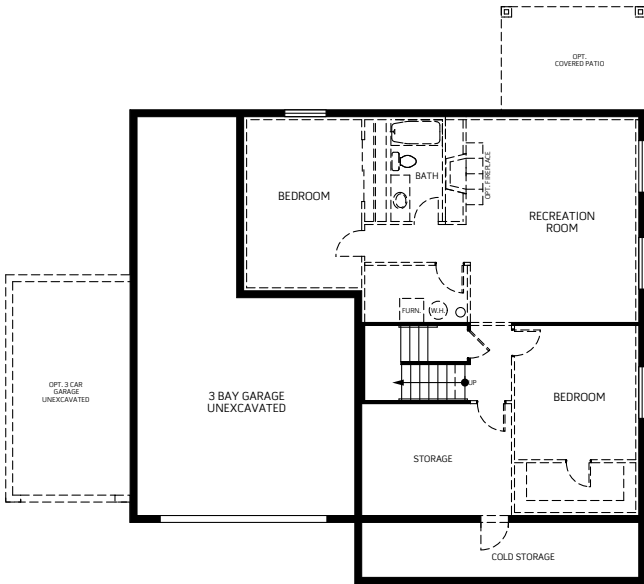
BASEMENT 1,227 Sq. Ft. Unfinished
