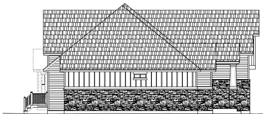
LEFT ELEVATION
