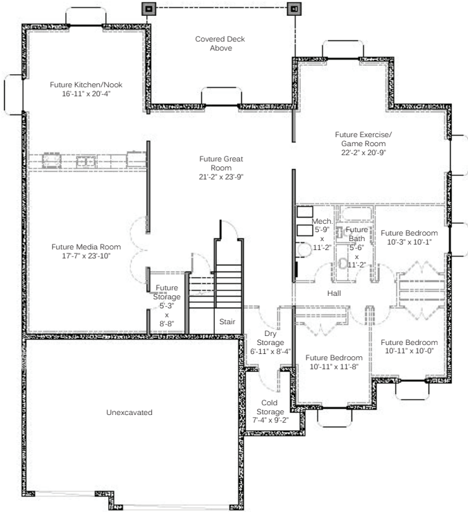
BASEMENT FLOOR
