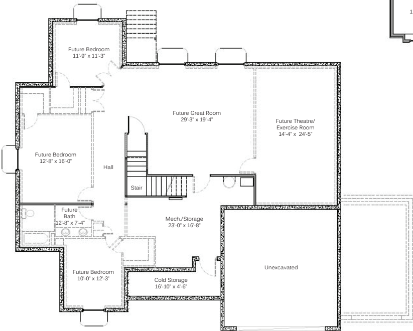
BASEMENT FLOOR
