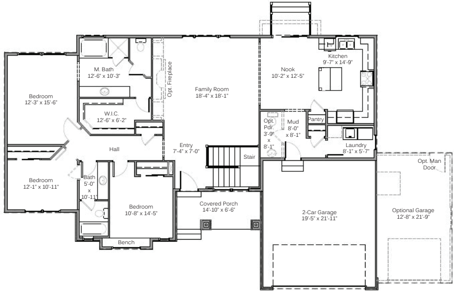
MAIN FLOOR
